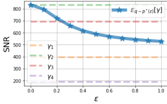
Fig. 6: Expected SNR of the communication link as \epsilon increases and the MTD scheme becomes more randomized. The SNR for each transmitter is also highlighted
